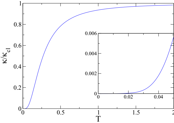
Fig. 1. Plot of the scaled thermal conductivity as a function of temperature (in units of \hbar\omega_c/k_B ) for \nu = 0.5 . Inset shows the low temperature behaviour.
