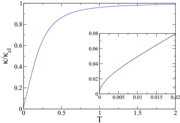
Fig. 2. Plot of the scaled thermal conductivity as a function of temperature (in units of \hbar\omega_c/k_B ) for \nu = 0.0 . Inset shows the low temperature behaviour.
